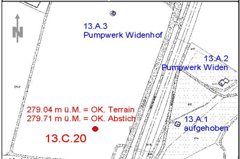
Situationsplan Arlesheim
